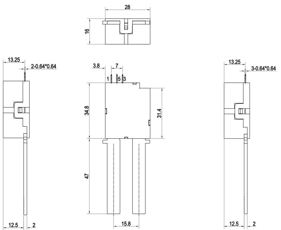
A type double coils
